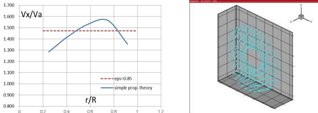
2.4. Figure 7 - Propeller slip stream obtained by axial momentum theory and Simple Propeller Theory
