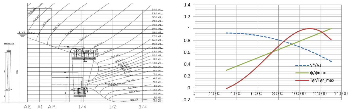
Fig.18 - After body and inflow data of Bulk Carrier Model
