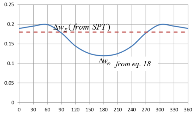
Figure 12 Effective wake change obtained from experiment (SPT) and calculation
