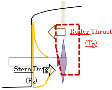
Figure 8. Representative interaction among stern, propeller and gate rudder
