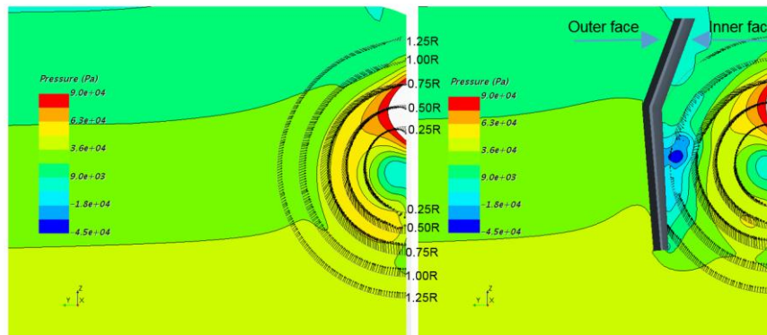
Figure 14. CFD computation of the flow field at actuator disc area with and without gate rudder (view from aft to fore and "R" is the propeller radius).
