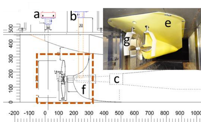
Figure 7. Measurement System of Emerson Cavitation Tunnel
